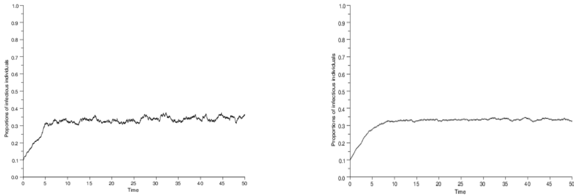
FIGURE 7. Realized trajectories of the modified \tau -leaping procedure for N = 2000 (left picture) and N = 20000 (right picture). The parameters are as in Figure 6.
