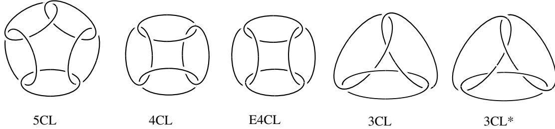
Figure 3: The minimally twisted 5-chain link 5CL, the 4-chain link 4CL, the minimally twisted 4-chain link E4CL and the 3-chain links 3CL and 3CL*. The exteriors of these links are respectively called M_5 , M_4 , F , M_3 and N .
