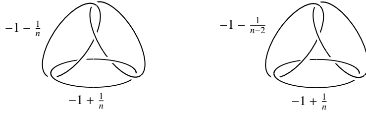
Figure 2: Surgery presentation for all (distinct) hyperbolic knots with a lens space and a toroidal filling at distance 3, or a lens space and a Seifert filling at distance 2, obtained by surgery on 5CL.
