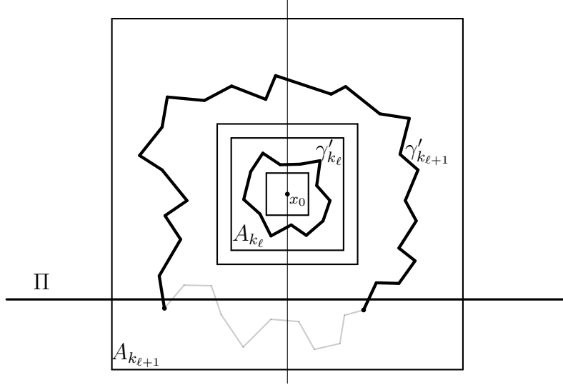
Figure 3: In the figure, the central vertex is x_0 ; around it, there are two cycles, \gamma_{k_\ell} and \gamma_{k_\ell+1} , positioned in the annuli A_{k_\ell} and A_{k_\ell+1} . Note that \gamma'_{k_\ell} = \gamma_{k_\ell} but \gamma'_{k_\ell+1} \subsetneq \gamma_{k_\ell+1} ( \gamma'_{k_\ell} and \gamma'_{k_\ell+1} are thickened while \gamma_{k_\ell+1} \setminus \gamma'_{k_\ell+1} is transparent). The proportions of the side lengths of the boxes, centered at x_0 , are not the real ones in the above schematic representation.
