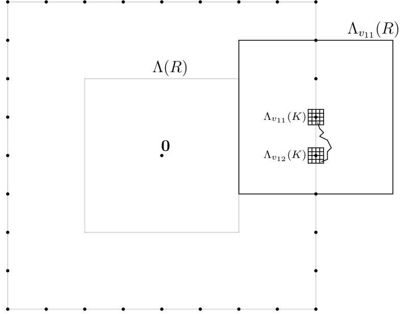
Figure 2: An illustration of the event described in (3) for i = 11 .
