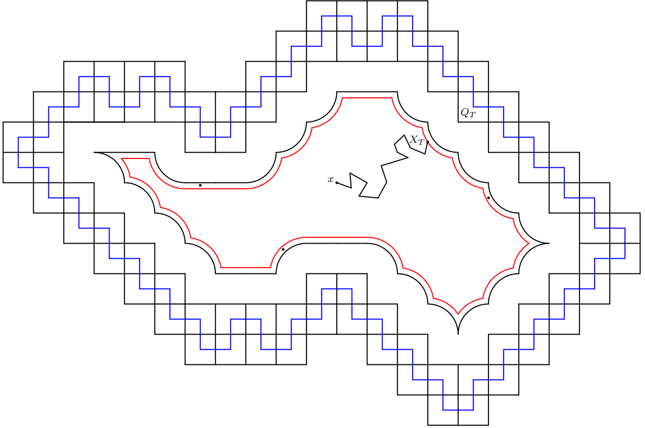
Figure 4: The figure depicts x , X_T and the square Q_T . The dominos in the cycle \mathcal{C}_1 are the ones intersecting the blue curve. The black contour corresponds to the boundary of \mathcal{C}_1^+ while the red contour is the boundary of B_T .
