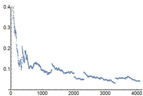
g = 4, \text{Err}(n)
