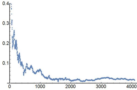
g = 2, \text{Err}(n)
