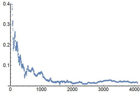
d = 1, \mathrm{Err}(n)
