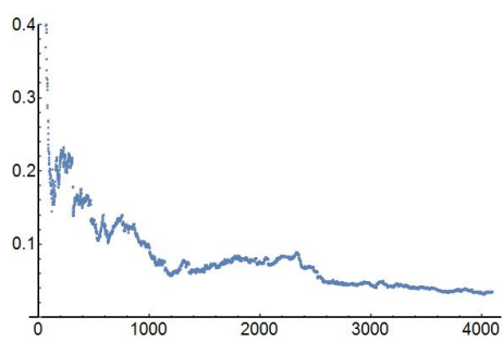
g = 3, \text{Err}(n)
