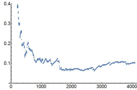
d = 2, \mathrm{Err}(n)
