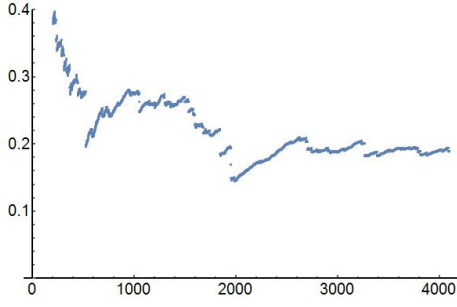
d = 3, \text{Err}(n)
