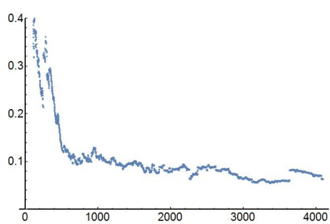
g = 5, \text{Err}(n)
