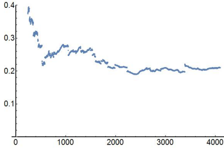
d = 5, \text{Err}(n)
