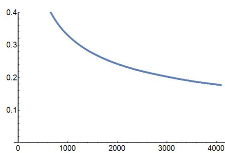
g = 5, \text{SErr}(n)
