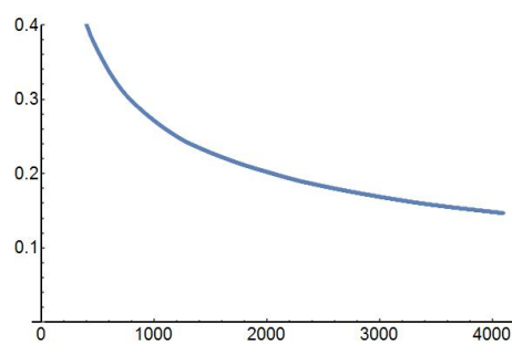
g = 4, \text{SErr}(n)
