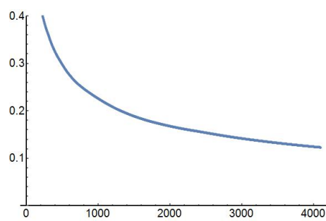
g = 3, \text{SErr}(n)
