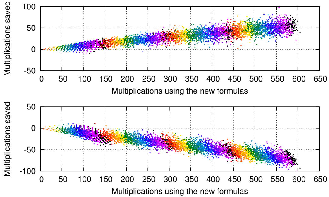
Fig. 7.2. Top: Points (x, y) for 100 randomly sampled b -bit integers n for each b \in \{2, 3, \dots, 64\} . Here x\mathbf{M} are used to compute P \mapsto nP on a twisted Hessian curve in projective coordinates; (x + y)\mathbf{M} are used to compute P \mapsto nP on a Weierstrass curve y^2 = x^3 - 3x + a_6 in Jacobian coordinates; and the color is a function of b . Bottom: Similar, but using a twisted Edwards curve rather than a Weierstrass curve.
