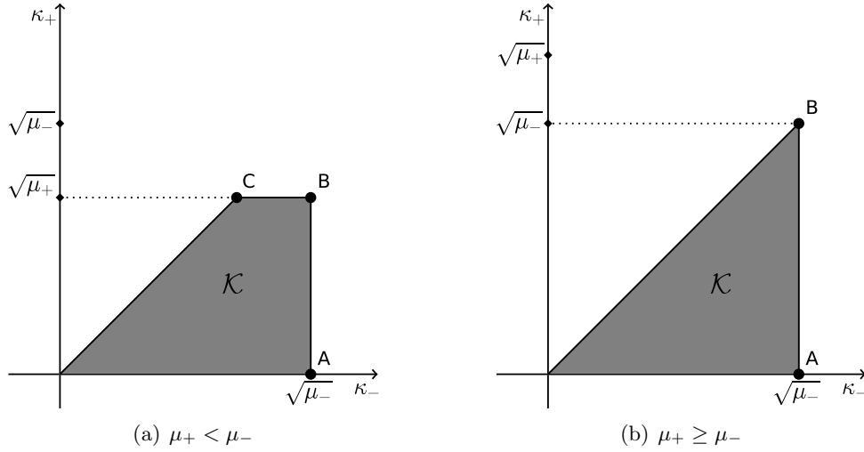
Figure 1: The set \mathcal{K} of admissible exponential decays.
