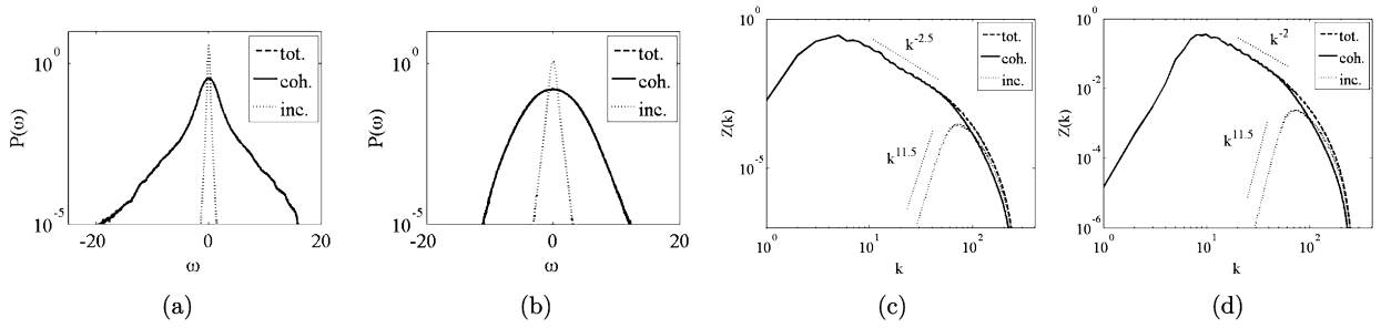
Fig. 4. POD results. (a, b): PDF of the vorticity. (c, d): wavenumber spectrum of the enstrophy. (a, c): quasi-hydrodynamic case. (b, d): quasi-adiabatic case. Dashed line: total field, solid line: coherent part, dotted line: incoherent part. Note that the coherent contribution (solid) superposes the total field (dashed), which is thus hidden under the solid line in all four figures. The straight lines indicating power laws are plotted for reference.
