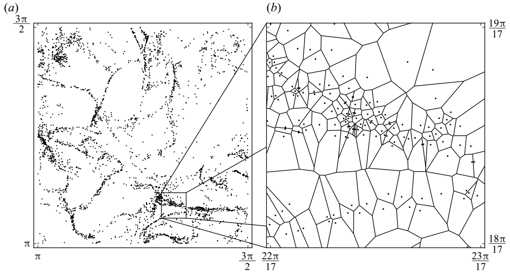
FIGURE 2. Voronoi tessellation generated by particles for St = 1 . Two-dimensional particle distribution in a slice of thickness 4\eta (a), corresponding to a zoom of figure 1(c). A magnified view with Voronoi tessellation (b).
