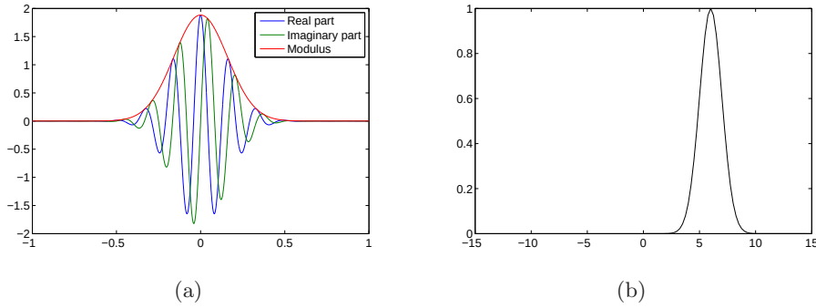
Figure 9: Localization of the Morlet wavelet in physical space (a) and in spectral space (b).
