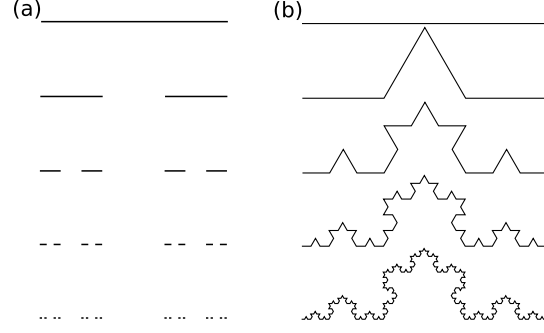
Figure 1: Illustration of the first four iteration steps leading to the Cantor dust (a) and to the von Koch snowflake (b).
