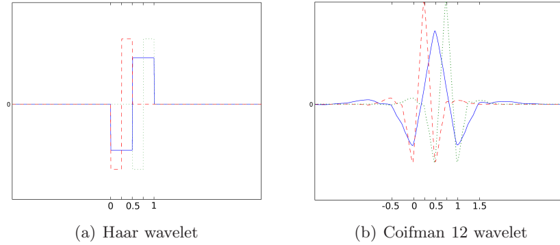
Figure 5: Orthogonal wavelets: Haar wavelet (left) and Coifman 12 wavelet (right). We have superposed one wavelet at scale j = 0 (blue) and position x = 0.5 ) and two wavelets at the next smaller scale j = 1 , located at position x = 0.25 (red) and x = 0.75 (green). They are mutually orthogonal, which can be directly seen for the Haar wavelet and which is much less obvious for the Coifman wavelet.
