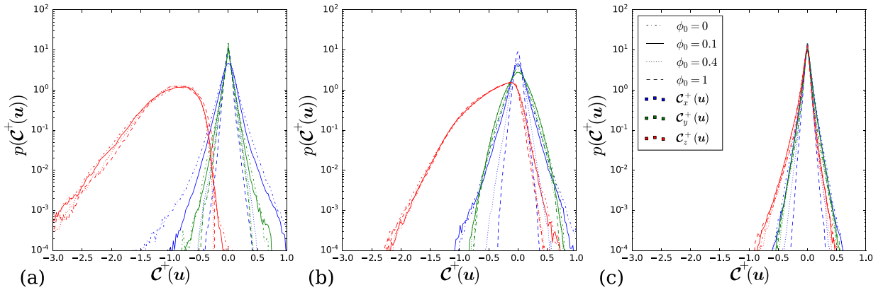
Fig. 3. PDF of fluid vorticity, normalised by the viscous time scale, for different mass loadings with Sr^+ = 7 , in the (a) viscous sublayer, (b) buffer layer and (c) log layer. The line colour indicates the component of the vorticity, and the line style indicates the mass loading.
