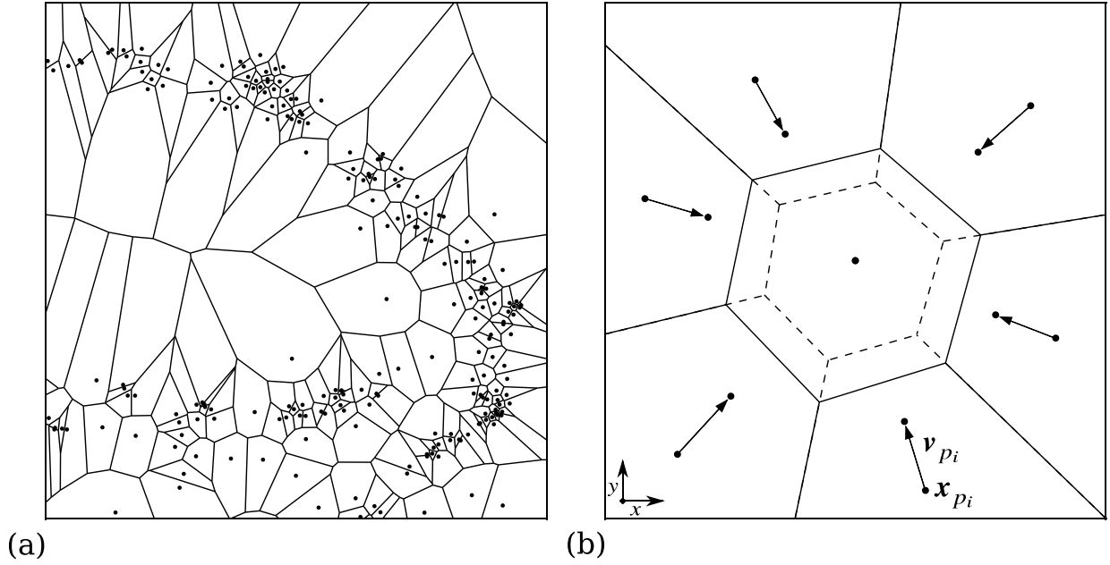
Fig. 1. (a) Voronoi tessellation in 2D for a cluster of particles. (b) Example of the motion of a two-dimensional modified Voronoi tessellation at two subsequent time instants for a converging cluster. The solid line corresponds to the time step t^k and the dashed line to t^{k+1} .
