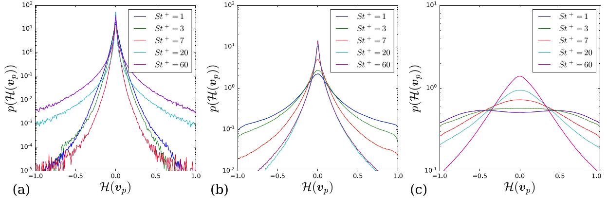
Fig. 14. PDFs of the relative helicity (cosine of the angle between particle velocity and vorticity) H(v_p) of the particles for various Stokes numbers with \phi_0 = 1 , in the (a) viscous sublayer, (b) buffer layer, and (c) log layer. Note that the y-ranges differ by orders of magnitude.
