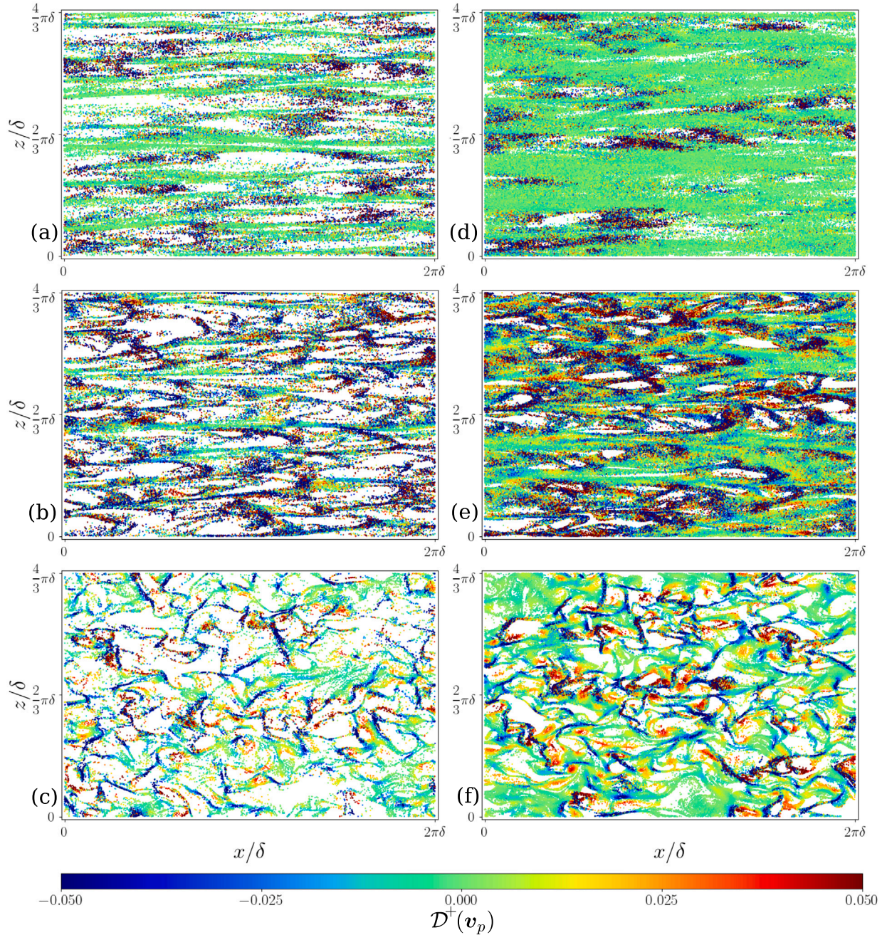
Fig. 15. Particle positions coloured by divergence in wall-parallel slices, for (a) viscous sublayer, \phi_0 = 0.1 , St^+ = 7 ; (b) buffer layer, \phi_0 = 0.1 , St^+ = 7 ; (c) log layer, \phi_0 = 0.1 , St^+ = 7 ; (d) viscous sublayer, \phi_0 = 0.4 , St^+ = 7 ; (e) buffer layer, \phi_0 = 0.4 , St^+ = 7 ; (f) log layer, \phi_0 = 0.4 , St^+ = 7 . Divergence is normalised by the viscous time scale, and the colour bar is truncated to emphasise regions of zero divergence. The slices used for visualisation are 2 \leq y^+ < 3 , 9.5 \leq y^+ < 14.5 and 97.5 \leq y^+ < 102.5 for viscous sublayer, buffer layer, and log layer, respectively.
