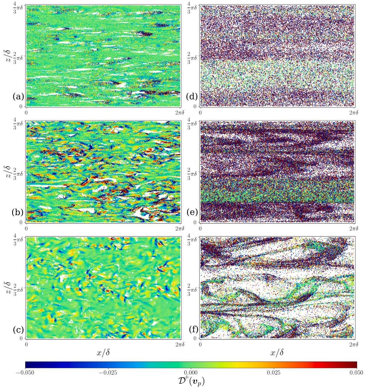
Fig. 7. Particle positions coloured by divergence in wall-parallel slices, for (a) viscous sublayer, Sr^+ = 3 , \phi_0 = 1 ; (b) buffer layer, Sr^+ = 3 , \phi_0 = 1 ; (c) log layer, Sr^+ = 3 , \phi_0 = 1 ; (d) viscous sublayer, Sr^+ = 60 , \phi_0 = 1 ; (e) buffer layer, Sr^+ = 60 , \phi_0 = 1 ; (f) log layer, Sr^+ = 60 , \phi_0 = 1 . Divergence is normalised by the viscous time scale, and the colour bar is truncated to emphasise regions of zero divergence. Because of the difference in number density, thinner slices are used to visualise the Sr^+ = 3 data. The slices used for Sr^+ = 3 are 2.375 \leq y^+ < 2.625 , 11.375 \leq y^+ < 12.625 and 99.375 \leq y^+ < 100.625 for viscous sublayer, buffer layer and log layer, respectively. The slices used for Sr^+ = 60 are 2 \leq y^+ < 3 , 9.5 \leq y^+ < 14.5 and 97.5 \leq y^+ < 102.5 for viscous sublayer, buffer layer and log layer, respectively.
