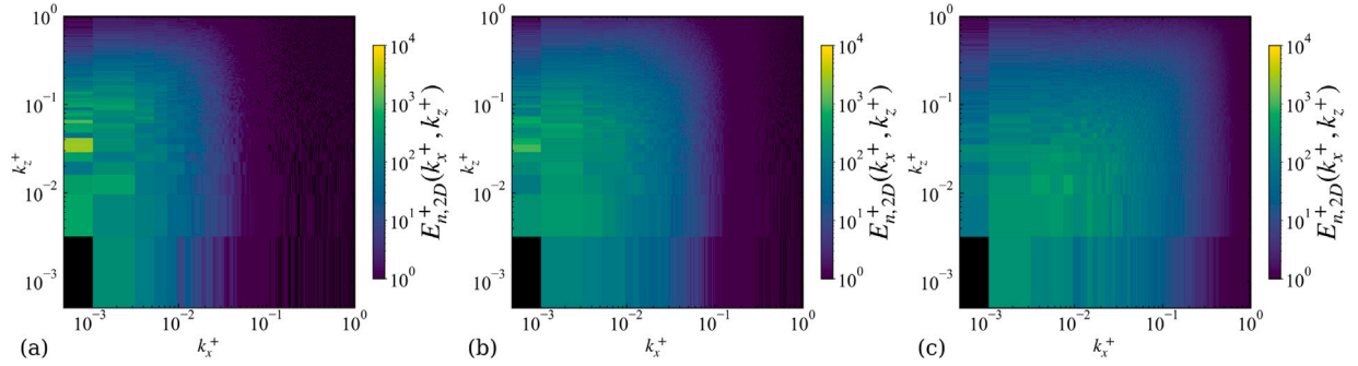
Fig. 24. 2D Fourier spectra of particle number density on 2D slices in (a) viscous sublayer, (b) buffer, and (c) log layers for \phi_0 = 1.0 and Sr^+ = 7 . The spectra and the wavenumber are normalised by the viscous length scale. Areas appearing in black indicate regions where there is no particle distribution.
