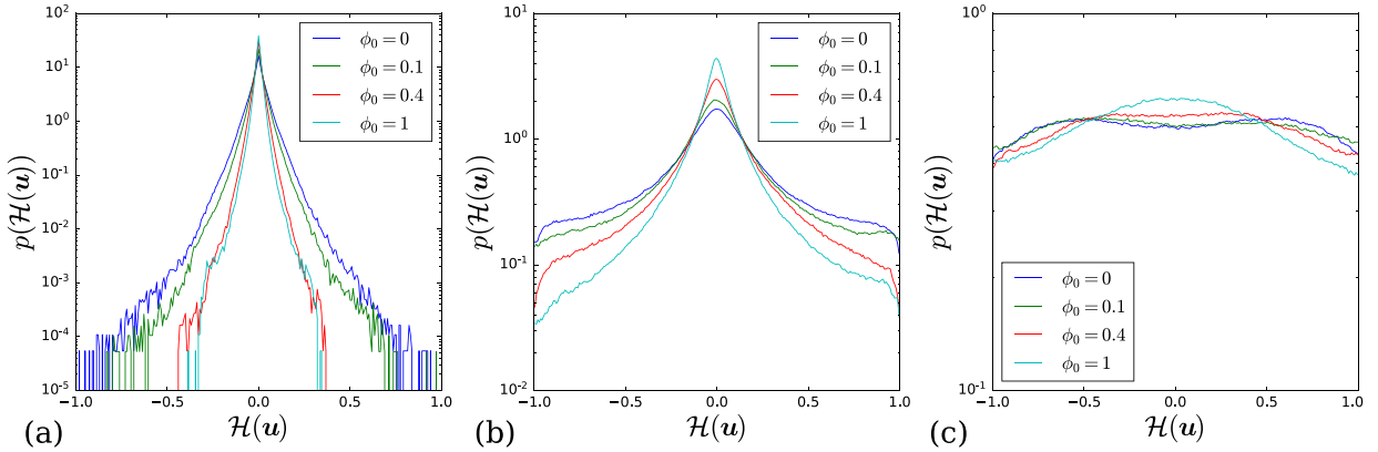
Fig. 5. PDF of fluid relative helicity for various mass loadings with Sr^+ = , in the (a) viscous sublayer, (b) buffer layer and (c) log layer. Note that the y-axis ranges for each PDF are different.
