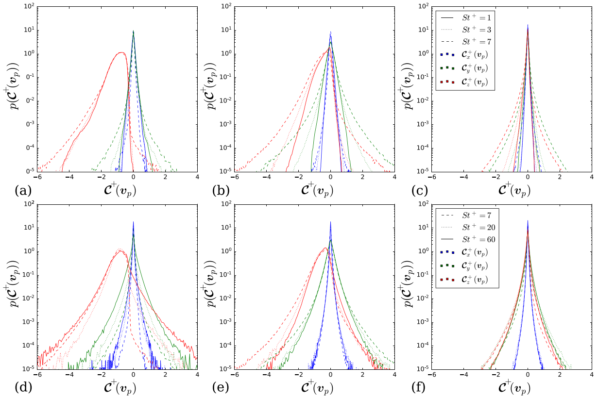
Fig. 13. PDF of particle velocity curl, normalised by the viscous time scale, for a range of Stokes numbers with \phi_0 = 1 . Data for small Stokes numbers: (a) viscous sublayer, (b) buffer layer and (c) log layer. Data for large Stokes numbers: (d) viscous sublayer, (e) buffer layer and (f) log layer. The line colour indicates the component of the curl, and the line style indicates the Stokes number.
