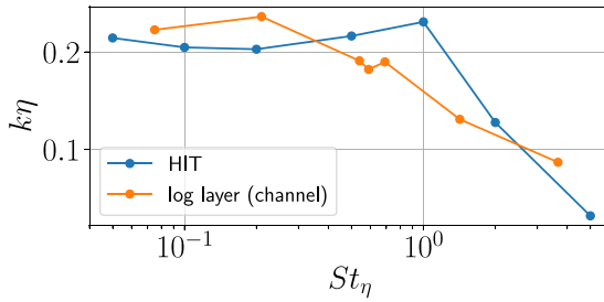
Fig. 22. Wavenumber of maximum in spectra of particle number density fluctuations as a function of Kolmogorov Stokes number for HIT (Matsuda et al., 2014) and the logarithmic layer in the present dataset.
