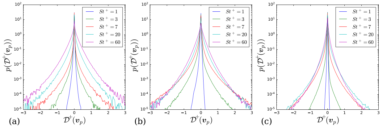
Fig. 11. PDF of particle velocity divergence, normalised by the viscous time scale, for various Stokes numbers with \phi_0 = 1 , in the (a) viscous sublayer, (b) buffer layer, and (c) log layer.
