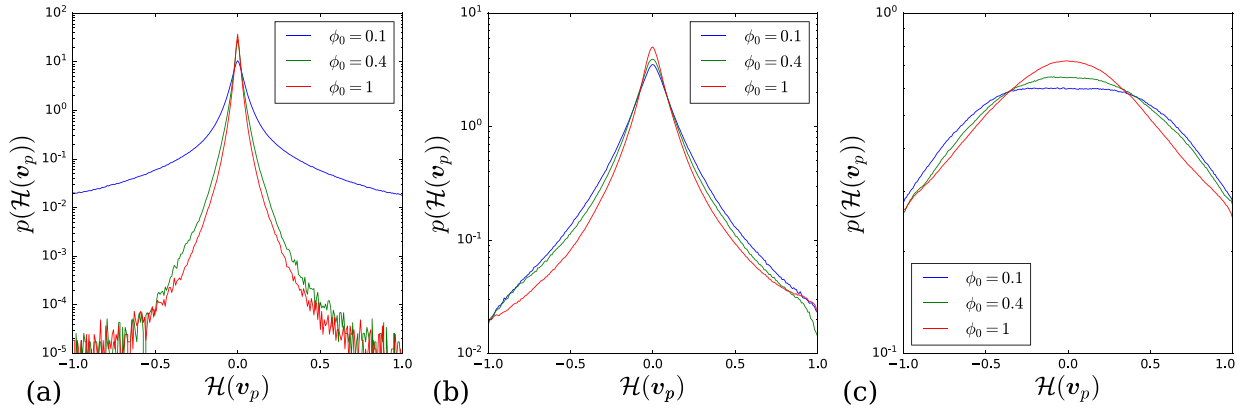
Fig. 19. PDFs of the relative helicity \mathcal{H}(\mathbf{v}_p) of the particles for different mass loadings with St^+ = 7 , in the (a) viscous sublayer, (b) buffer layer and (c) log layer. Note that the y-ranges differ by orders of magnitude.
