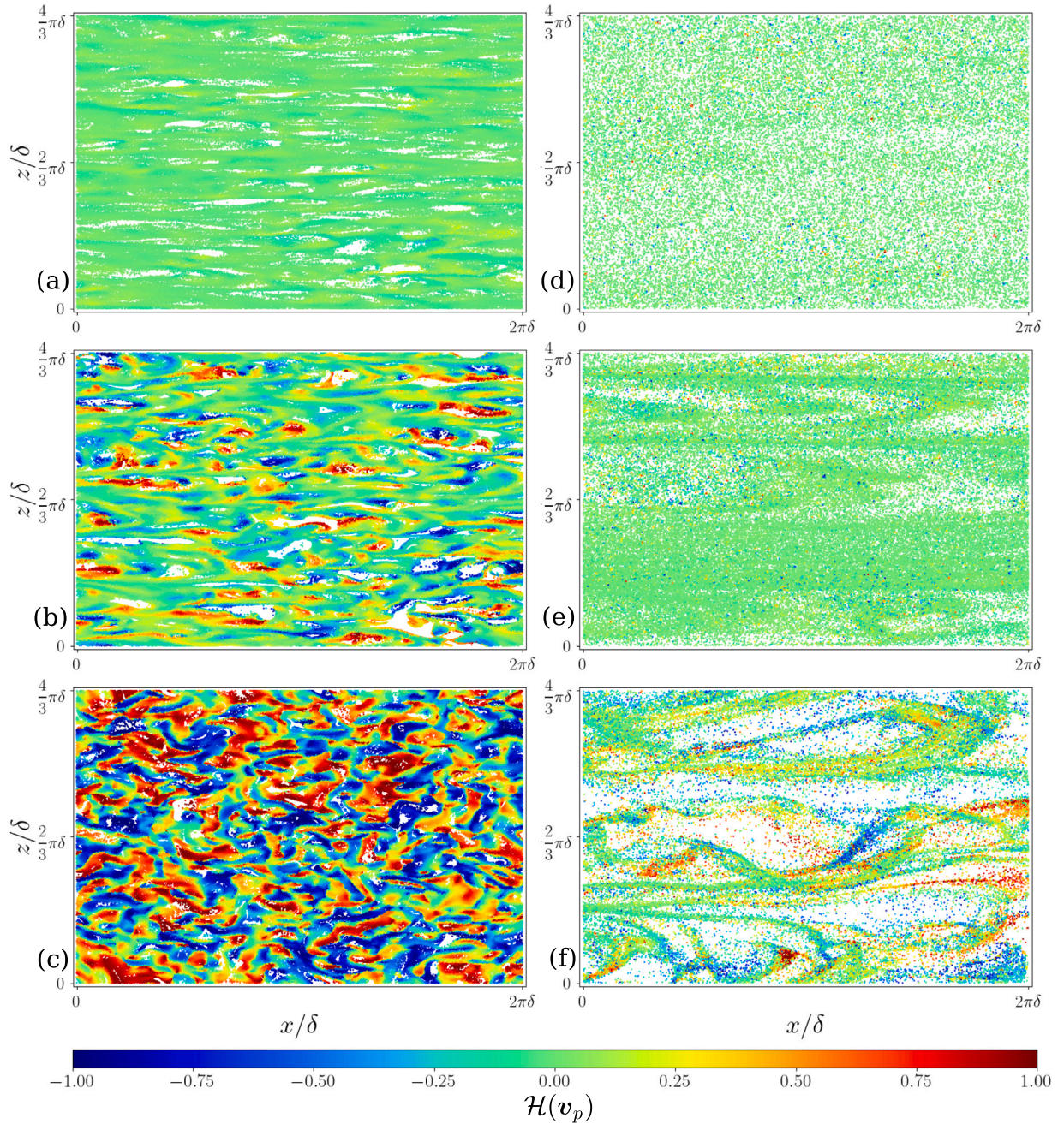
Fig. 9. Particle positions coloured by relative helicity in wall-parallel slices, for (a) viscous sublayer, St^+ = 3 , \phi_0 = 1 ; (b) buffer layer, St^+ = 3 , \phi_0 = 1 ; (c) log layer, St^+ = 3 , \phi_0 = 1 ; (d) viscous sublayer, St^+ = 60 , \phi_0 = 1 ; (e) buffer layer, St^+ = 60 , \phi_0 = 1 ; (f) log layer, St^+ = 60 , \phi_0 = 1 . Thickness of the layers used are defined in Fig. 7.
