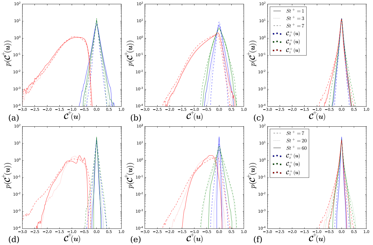
Fig. 4. PDF of fluid vorticity, normalised by the viscous time scale, for a range of Stokes numbers with \phi_0 = 1 . Data for small Stokes numbers: (a) viscous sublayer, (b) buffer layer and (c) log layer. Data for large Stokes numbers: (d) viscous sublayer, (e) buffer layer and (f) log layer. The line colour indicates the component of the vorticity, and the line style indicates the Stokes number.
