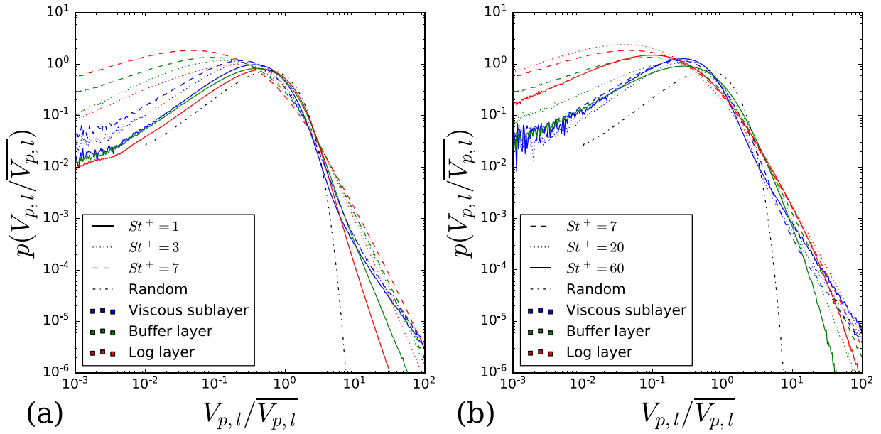
Fig. 10. PDF of modified Voronoi volume as a function of flow region and Stokes number, normalised by the mean modified Voronoi volume within each layer for (a) St^+ = 1, 3, 7 ; \phi_0 = 1 , and (b) St^+ = 7, 20, 60 ; \phi_0 = 1 . The dashed-dotted line represents the volume distribution for randomly distributed particles.
