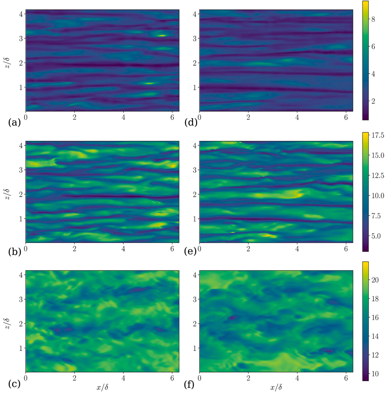
Fig. 25. Fluid streamwise velocity u^+ for (a) \phi_0 = 0.1 , Sr^+ = 7 at y^+ = 2.5 ; (b) \phi_0 = 0.1 , Sr^+ = 7 at y^+ = 12 ; (c) \phi_0 = 0.1 , Sr^+ = 7 at y^+ = 100 ; (d) \phi_0 = 0.4 , Sr^+ = 7 at y^+ = 2.5 ; (e) \phi_0 = 0.4 , Sr^+ = 7 at y^+ = 12 ; (f) \phi_0 = 0.4 , Sr^+ = 7 at y^+ = 100 .
