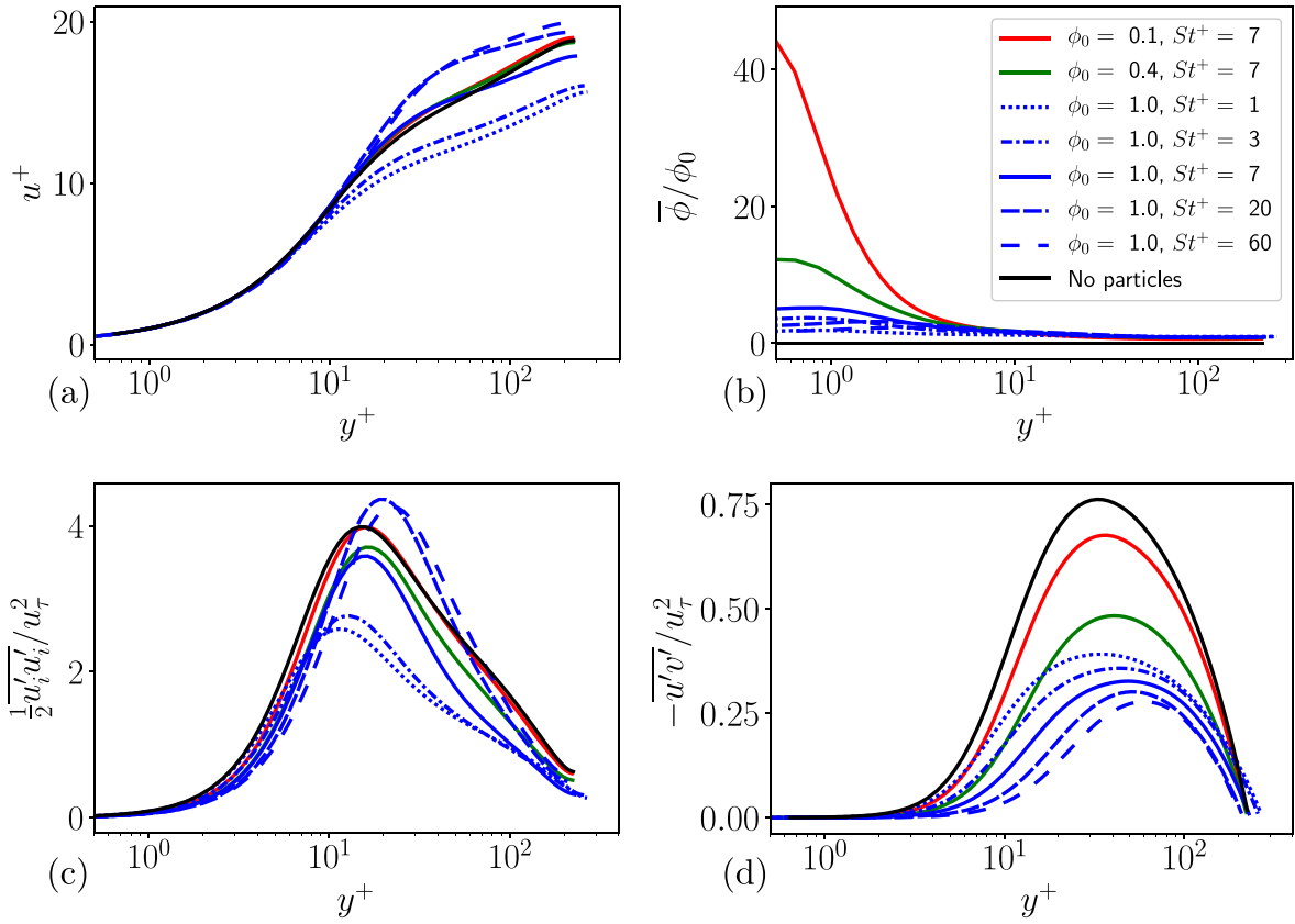
Fig. 2. (a) Mean streamwise fluid velocity, u^+ , as a function of wall-normal distance, y^+ , for various mass loadings and Stokes numbers, as well as without particles. (b) Local mean mass loading. (c) Fluid phase turbulent kinetic energy (TKE). (d) Fluid phase Reynolds shear stress ( u'v' ). The legend in (b) applies to all sub-figures.
