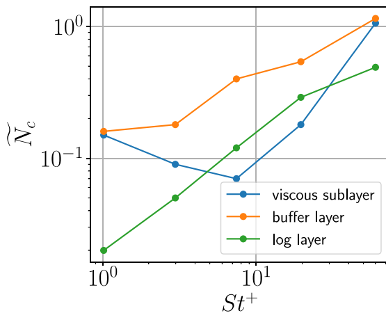
Fig. 12. Collision rate non-dimensionalised according to Eq. (15) for various Stokes numbers with \phi_0 = 1 .
