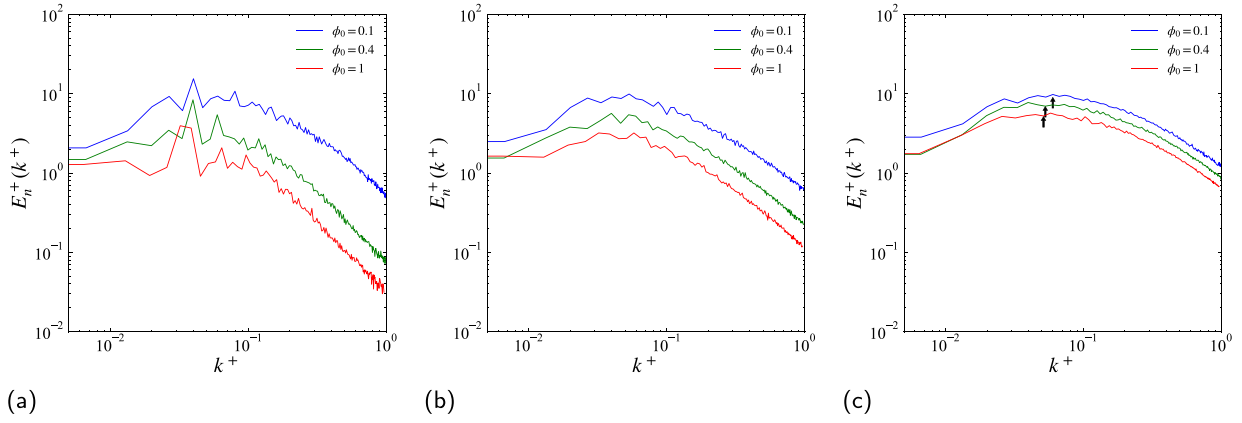
Fig. 23. Fourier spectra of particle number density on 2D slices in (a) viscous sublayer, (b) buffer, and (c) log layers for various mass loadings with Sr^+ = 7 . The spectra and the wavenumber are normalised by the viscous length scale. In (c), the peak locations obtained with a five-point moving average are indicated with arrows.
