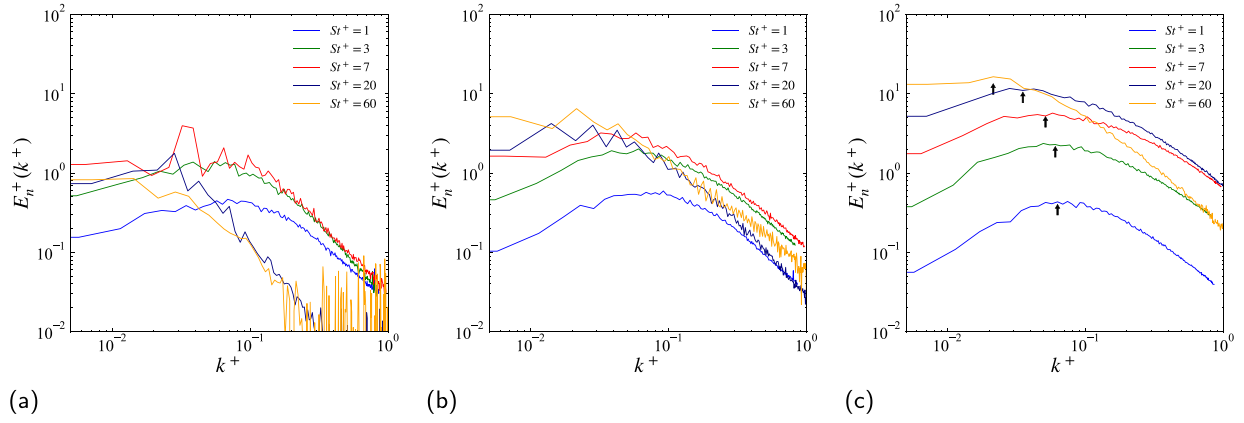
Fig. 21. Fourier spectra of particle number density in 2D slices in (a) viscous sublayer, (b) buffer, and (c) log layers for various Stokes numbers with \phi_0 = 1 . The spectra and the wavenumber are normalised by the viscous length scale. In (c), the peak locations obtained with a five-point moving average are indicated with arrows.
