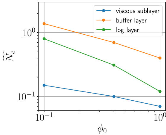
Fig. 17. Collision rate non-dimensionalised according to Eq. (15) for various mass loadings with Sr^+ = 7 .
