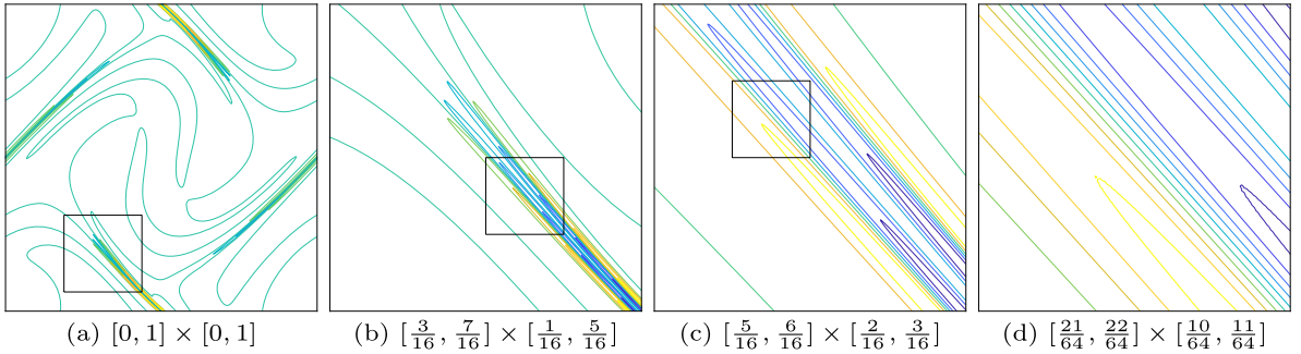
Fig. 8. Gradual 64 \times zoom on the Laplacian of the vorticity at t = 4 .
