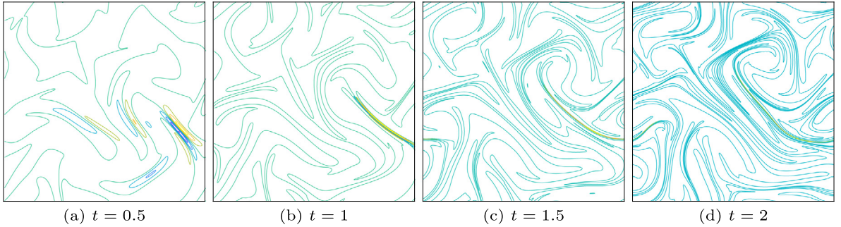
Fig. 13. Contour plot of \Delta \omega^n for the random initial condition test using 256^2 grid for \mathcal{X}^n , 1024^2 grid for representing \psi^n , \Delta t = 1/128 and \delta_{\text{det}} = 10^{-4} .
