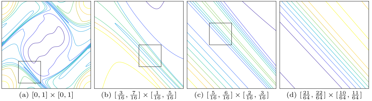
Fig. 7. Gradual 64 \times zoom on the vorticity at t = 4 .
