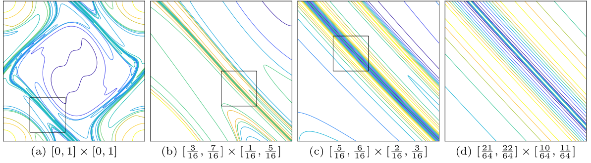
Fig. 9. Gradual 64 \times zoom on the vorticity at t = 8 .
