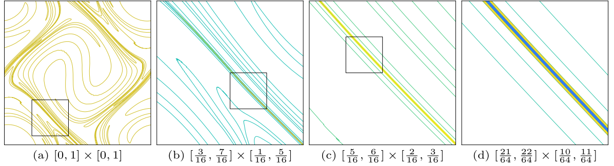
Fig. 10. Gradual 64 \times zoom on the Laplacian of the vorticity at t = 8 .
