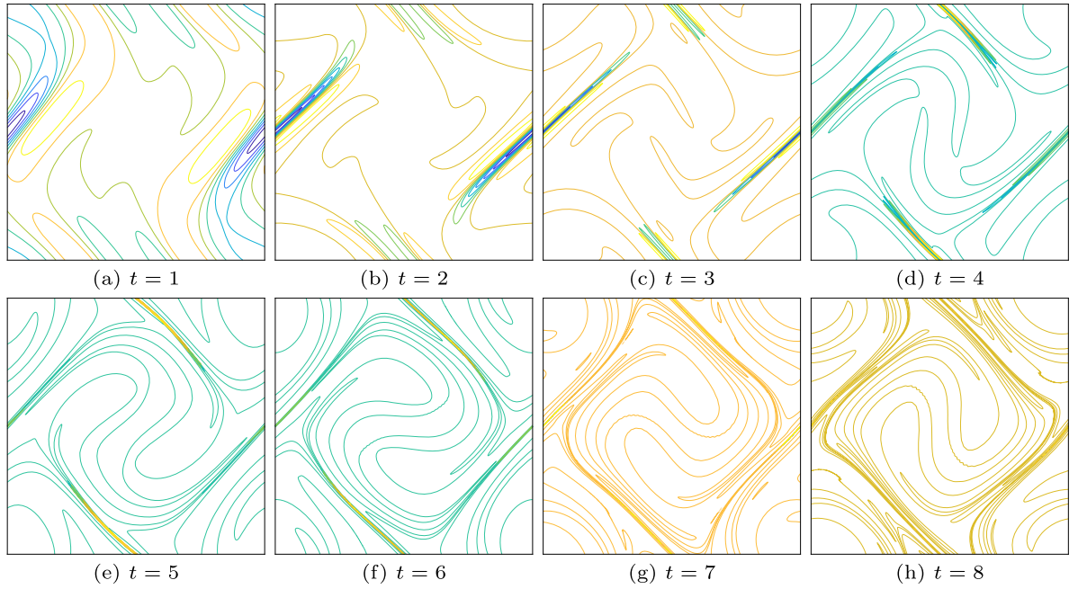
Fig. 6. Contour plot of the Laplacian of the vorticity using 128^2 grid for \mathcal{X}^n , 512^2 grid for representing \psi^n , \Delta t = 1/32 and \delta_{\text{det}} = 10^{-4} .
