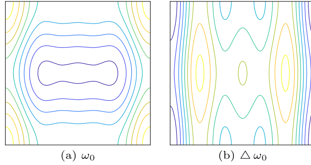
Fig. 4. Contour plot of the 4-modes initial vorticity and its Laplacian. Isolines are shown for 9 values uniformly distributed in the range of each function.
