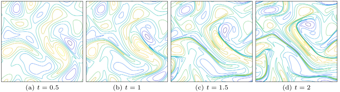
Fig. 12. Contour plot of \omega^n for the random initial condition test using 256^2 grid for \mathcal{X}^n , 1024^2 grid for representing \psi^n , \Delta t = 1/128 and \delta_{\text{det}} = 10^{-4} .
