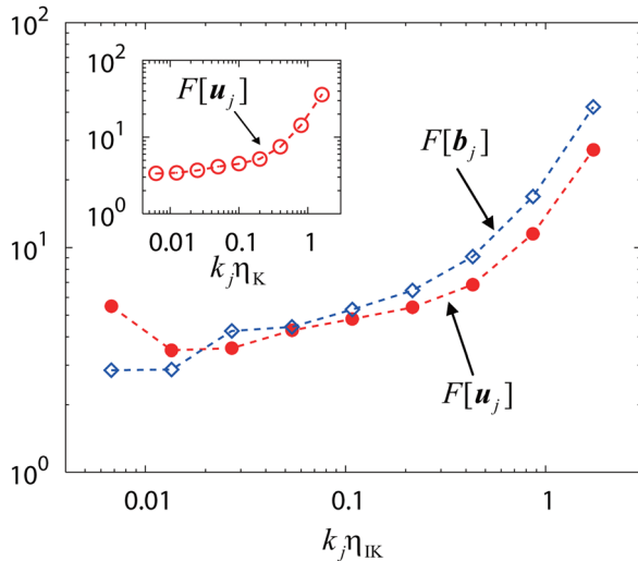
FIG. 3. (Color online) Scale-dependent flatness of velocity and magnetic field, F[\mathbf{u}_j] and F[\mathbf{b}_j] , vs. k_j \eta_{ik} for MHD turbulence. The inset shows F[\mathbf{u}_j] vs. k_j \eta_K for HD turbulence.
