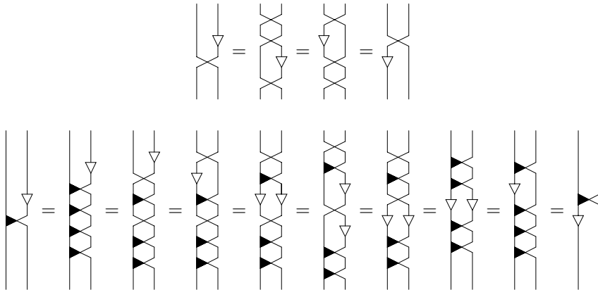
Figure 43: Deriving rules for \mathbf{GA}(\mathbb{Z}_2)
