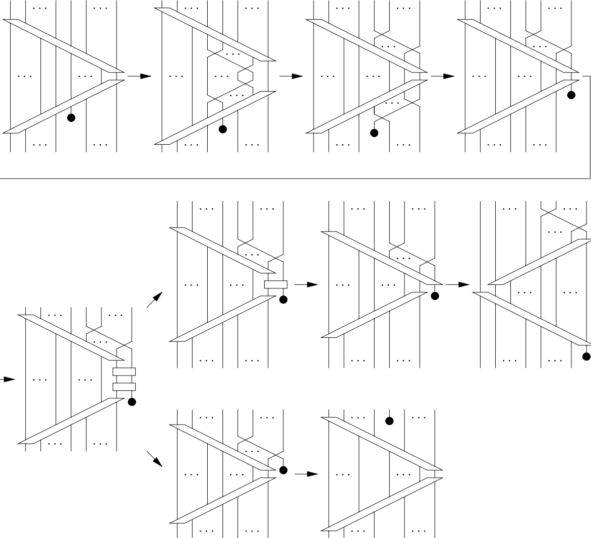
Figure 32: Crucial transformation for \mathbf{L}^{\text{surj}}(\mathbb{Z}_2)
