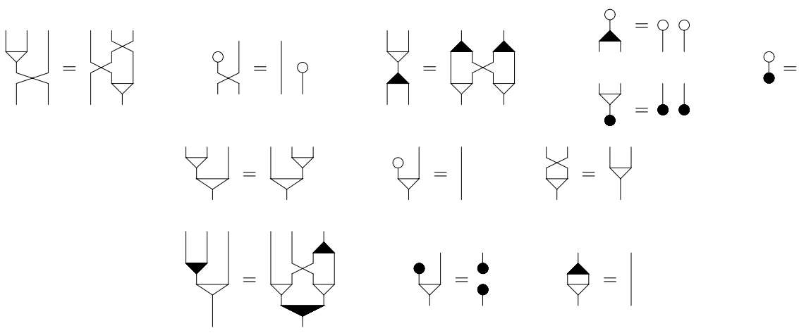
Figure 40: Extra relations for \mathfrak{F}[2]
