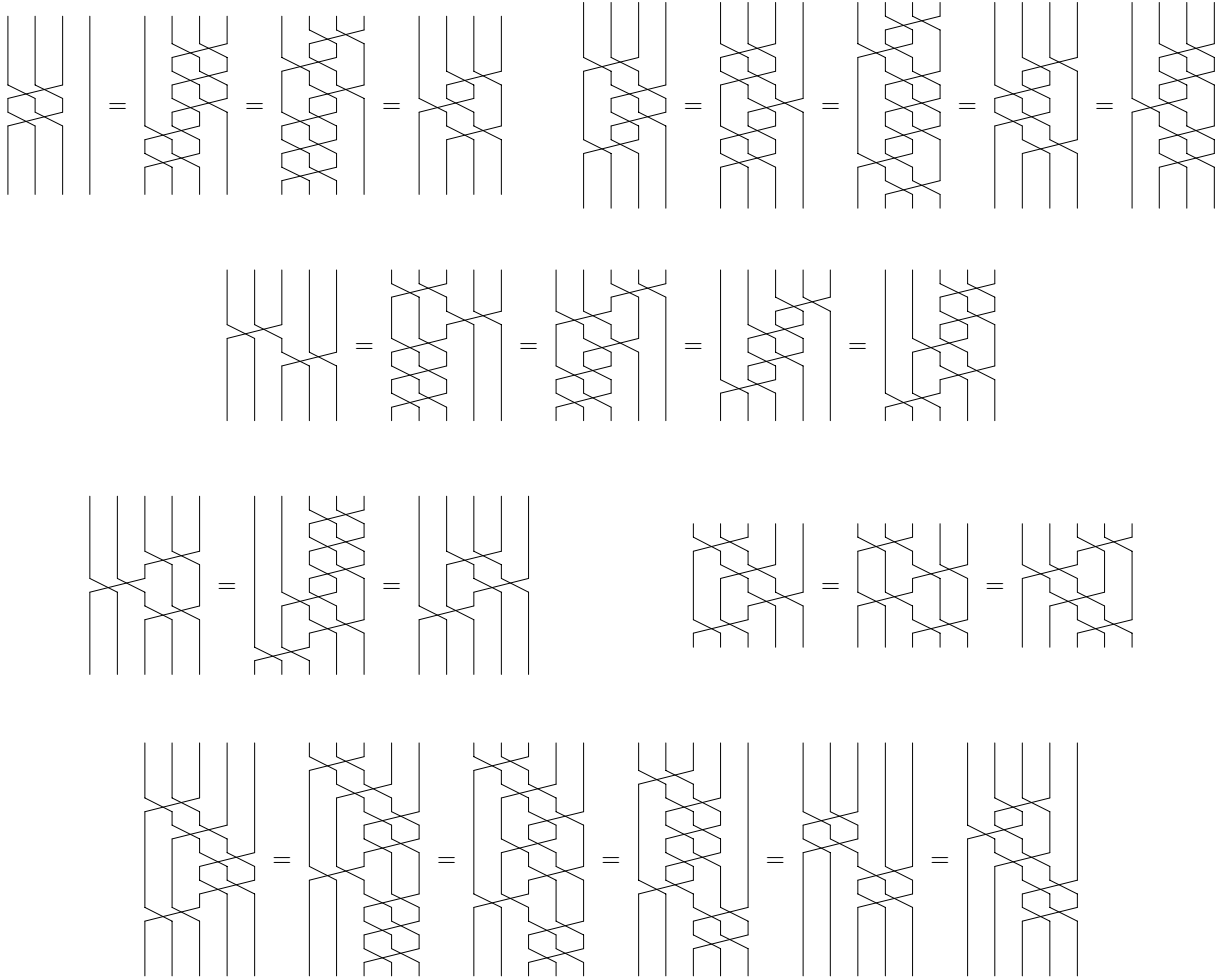
Figure 11: Deriving rules for \mathfrak{A}
