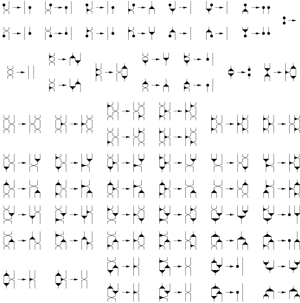
Figure 28: Alternative rules for \mathbf{L}(\mathbb{Z}_2)
