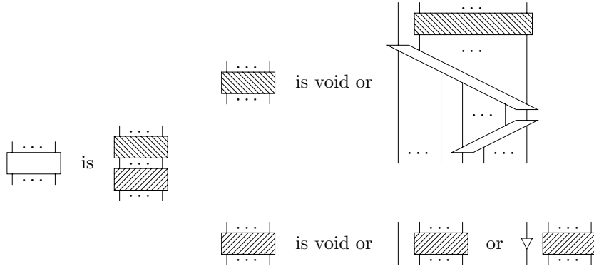
Figure 41: Canonical form for \mathbf{GA}(\mathbb{Z}_2)
