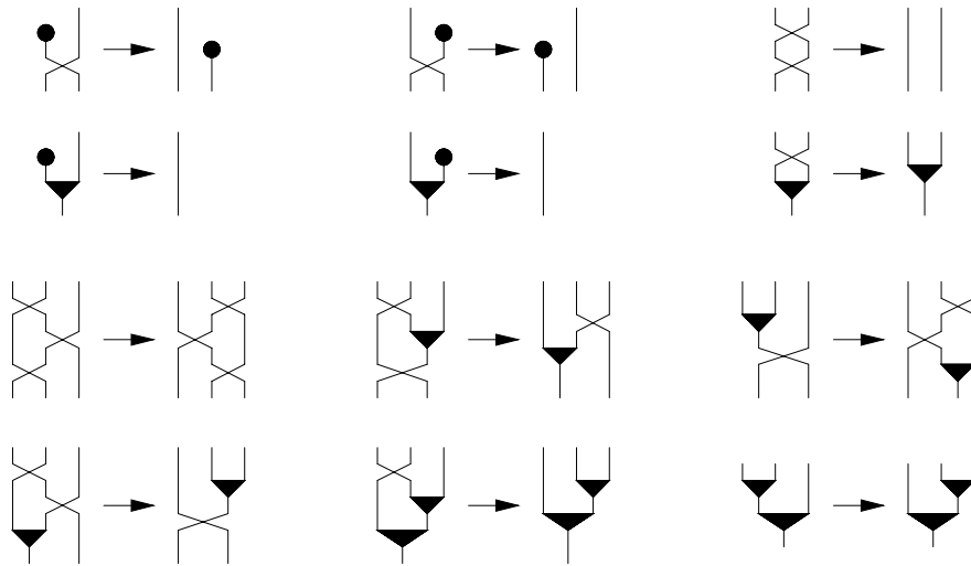
Figure 9: Alternative rules for \mathfrak{F}
