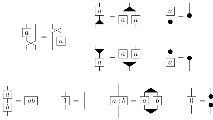
Figure 36: Extra relations for \mathbf{L}(K)
