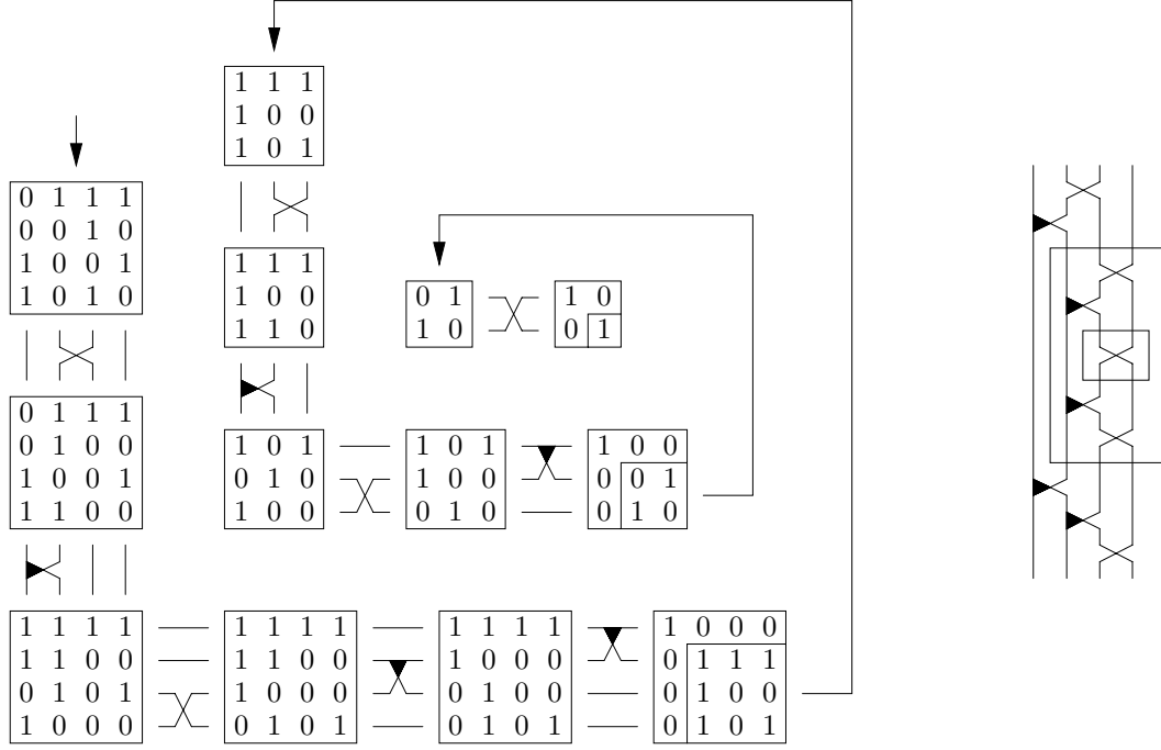
Figure 16: Computing the first canonical form of a matrix in \mathbf{GL}(\mathbb{Z}_2)
