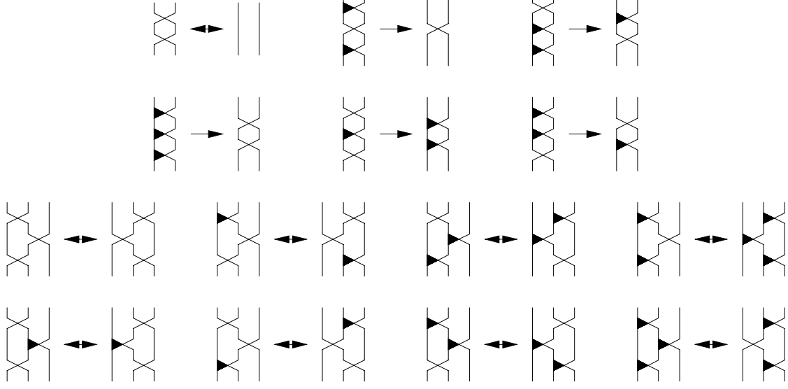
Figure 18: Rules for \mathbf{GL}(\mathbb{Z}_2)
