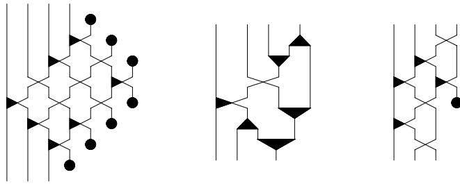
Figure 23: The canonical forms of a matrix in \mathbf{L}(\mathbb{Z}_2)
