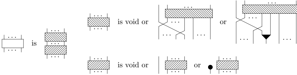
Figure 8: Alternative canonical form for \mathfrak{F}
