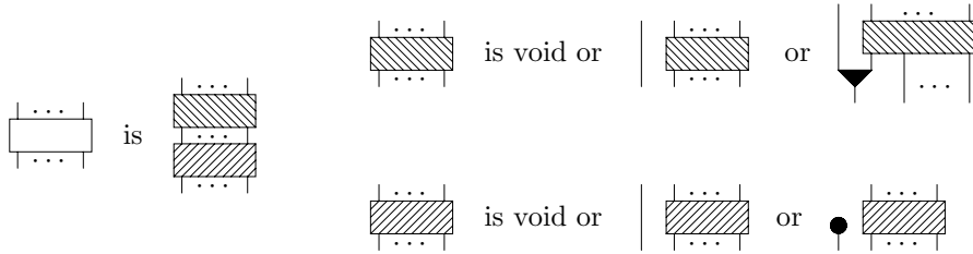
Figure 3: Alternative canonical form for \mathfrak{M}
