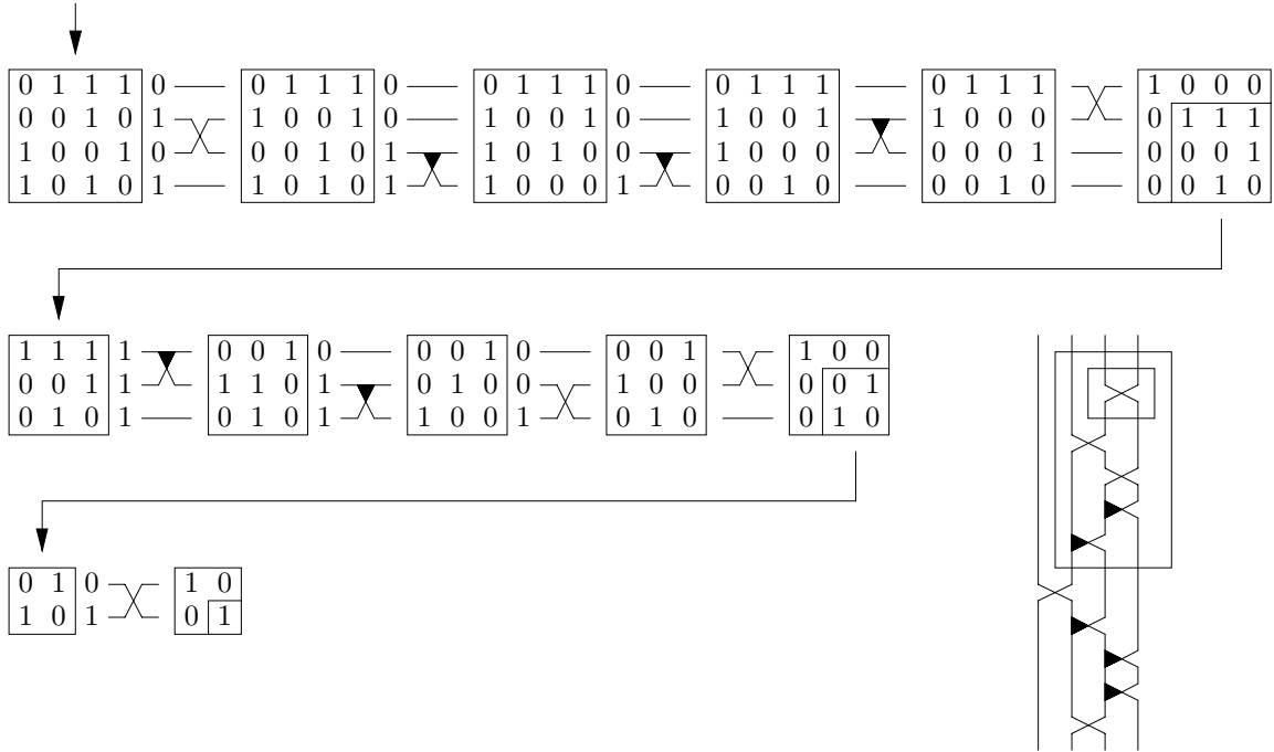
Figure 17: Computing the second canonical form of a matrix in \mathbf{GL}(\mathbb{Z}_2)
