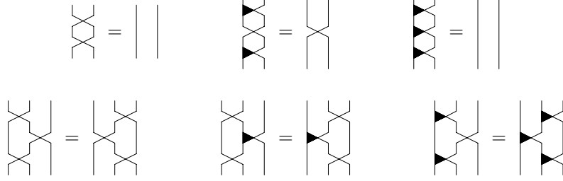
Figure 15: Relations for \mathbf{GL}(\mathbb{Z}_2)
