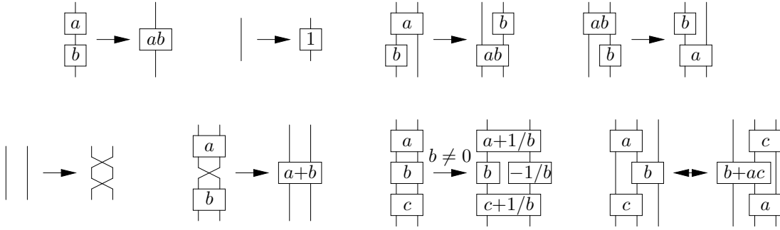
Figure 37: Rules for \mathbf{GL}(K)
